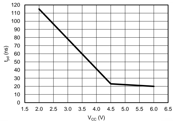
Figure 5. Propagation Delay vs Supply Voltage at T_A = 25^\circ\text{C}
