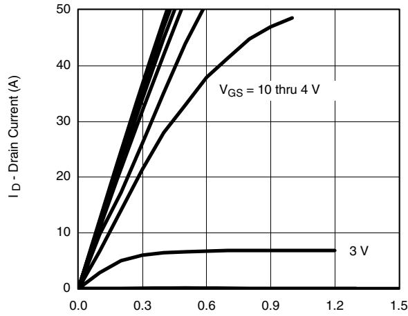
V_{GS} = 10 thru 4 V 3 V Output Characteristics
