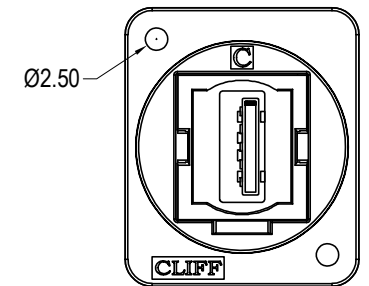
'X' VERSION \varnothing 2.5 PLAIN HOLES
