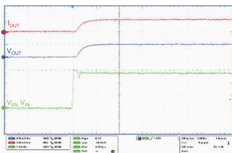
Figure 39. Turn-on time
