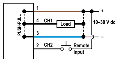
Figure 3. Channel 1 as a Push-Pull discrete output, Channel 2 as remote input
