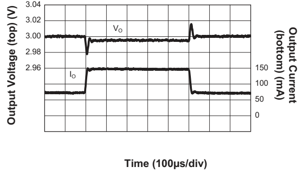
Load Transient Response LDO4 ( I_{OUT4} = 75mA to 150mA ; V_{BAT} = 3.6V ; V_{OUT4} = 3V ; C_{OUT} = 4.7\mu F )
