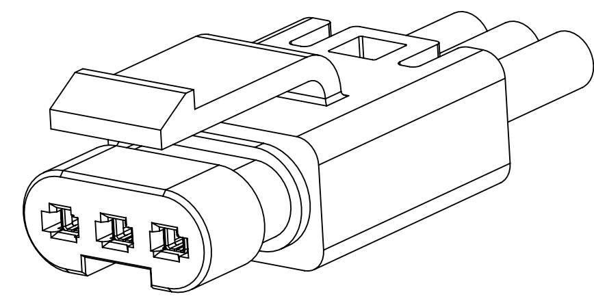
END CONNECTOR ASSEMBLY WITH 3 CONTACTS CRIMPED TO WIRES AND INSTALLED
