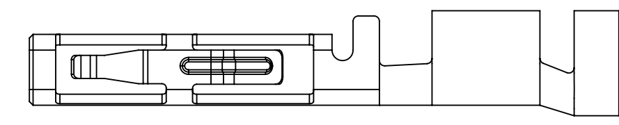
FLH-SC136-1-XXX - SOCKET CONTACT SEE NOTES 3 & 5 SCALE 10:1
