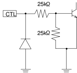
CTL Pin
