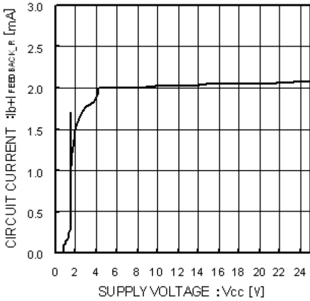
Fig.2 Circuit Current
