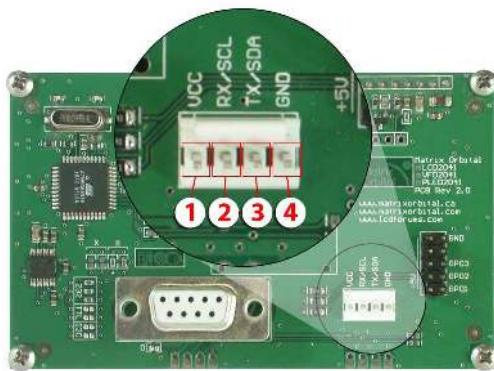
Figure 15: Power Connector and Pin out
