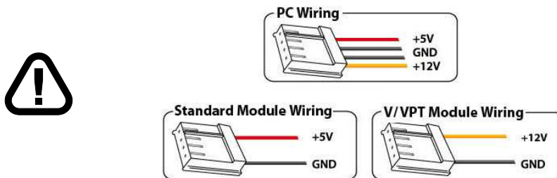
Figure 10: PC vs Matrix Orbital Display Module Wiring
