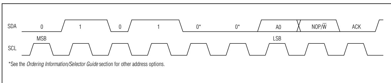
Figure 4. Slave Address
