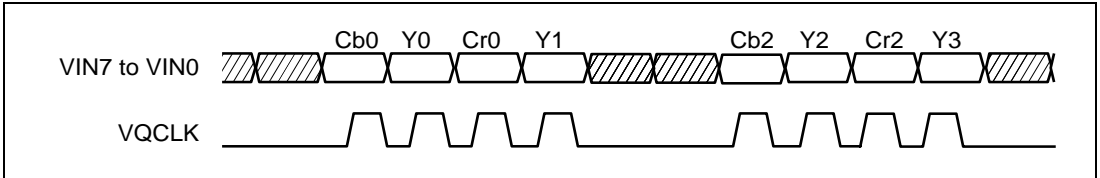
Figure 3.51 Video Incorporation Signals
