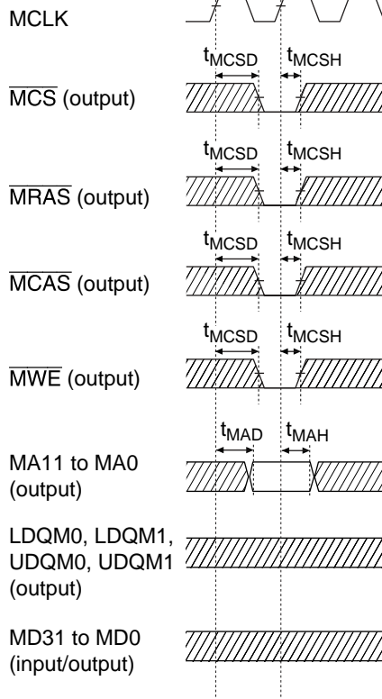
Figure 7.11 (2) UGM Mode Register Setting Cycle Timing
