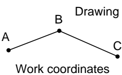
Figure 3.38 Drawing Functions
