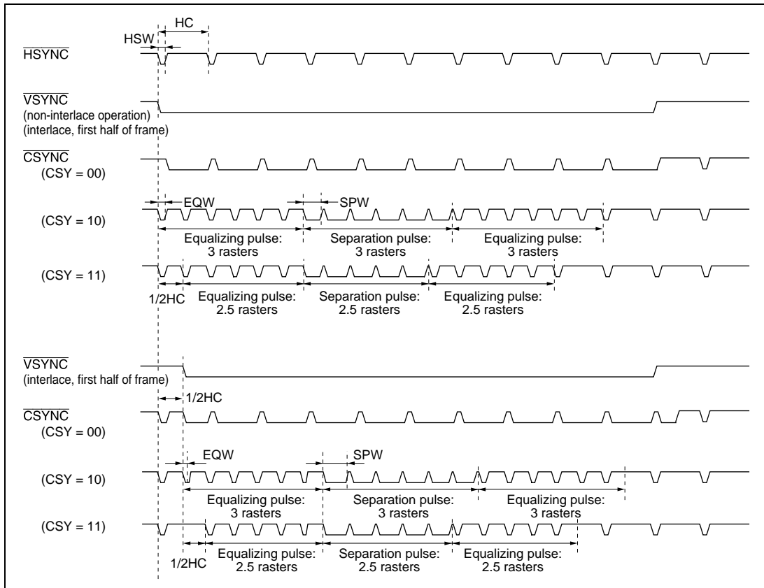
Figure 3.37 CSYNC Output Waveform
