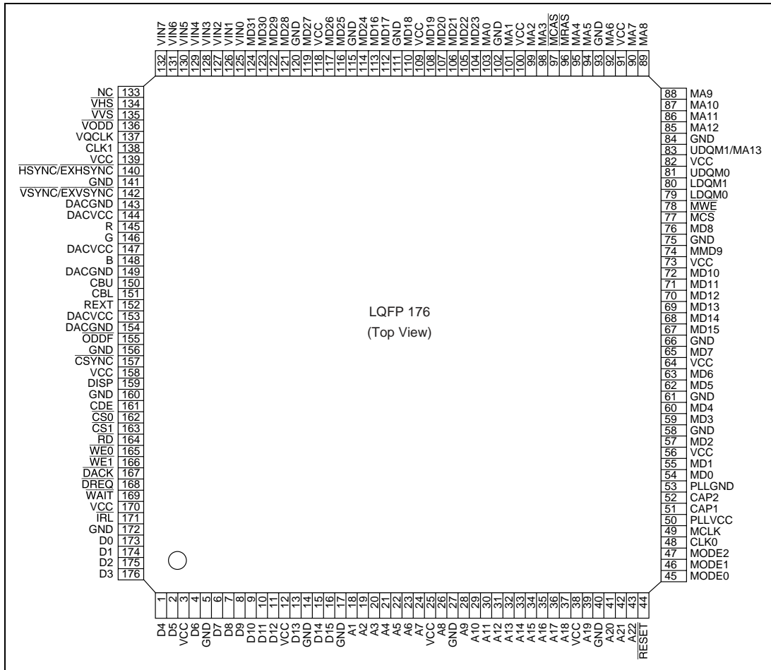
Figure 2.2 Pin Arrangement
