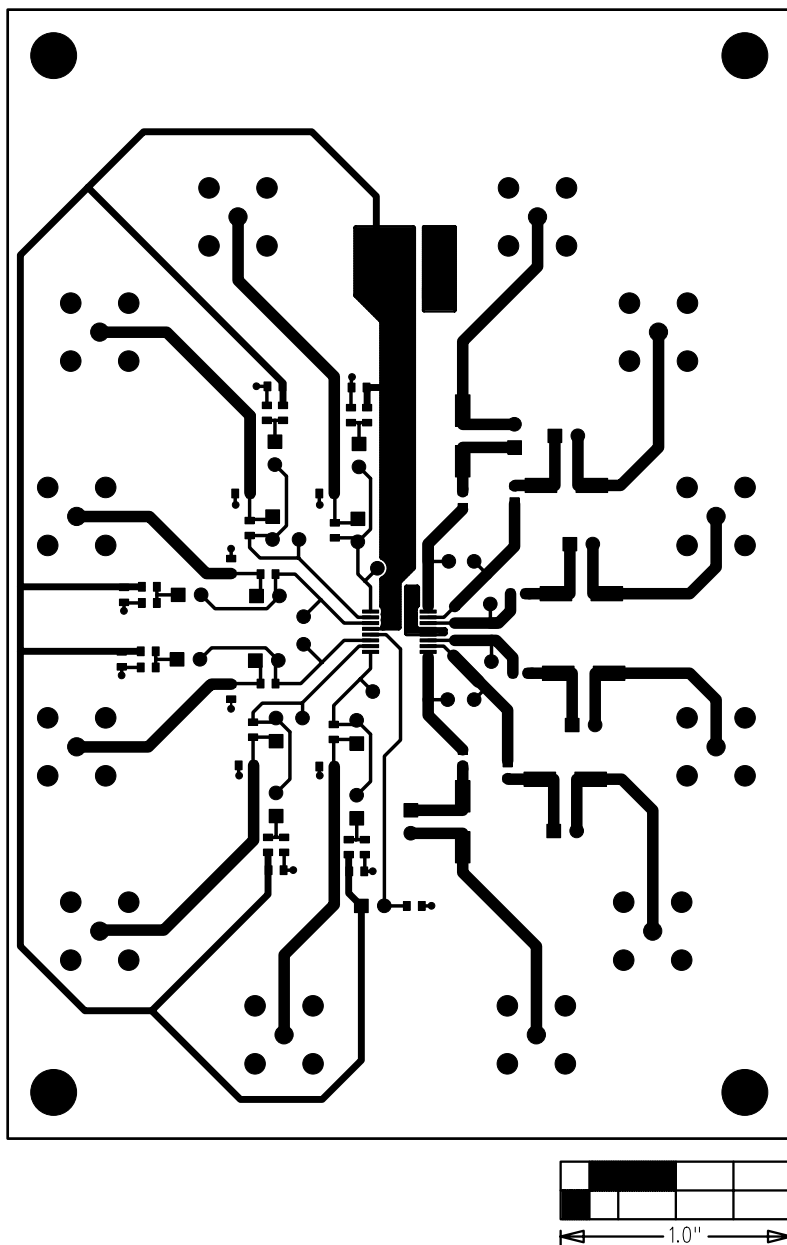
Figure 3. MAX11506 EV Kit PCB Layout—Component Side
