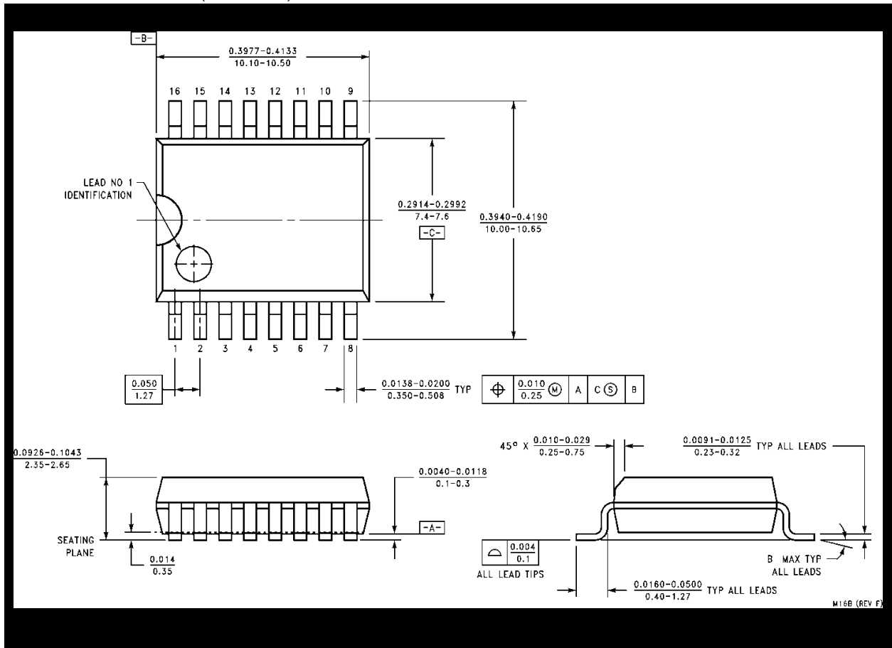
Figure 13. 16-Lead Small Outline Intergrated Circuit (SOIC), JEDEC MS-013, 0.300" Wide Package Number M16B
