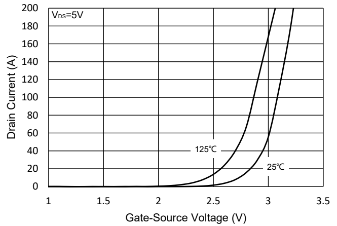
Fig.2 Transfer Characteristic
