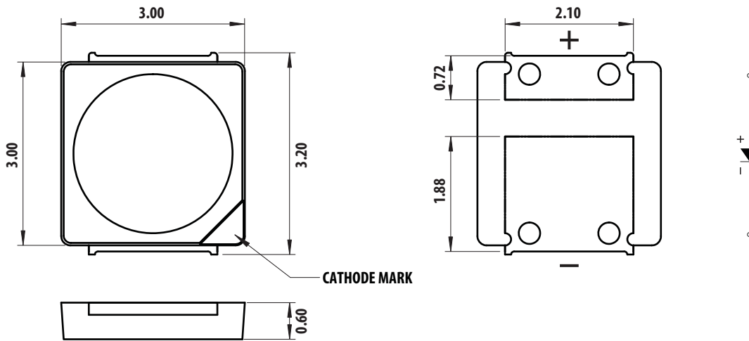
Figure 1: Package Drawing
