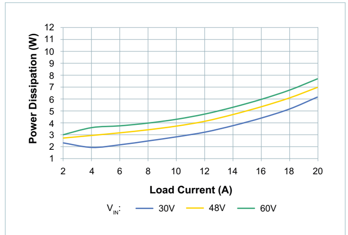
Figure 43 — System Power Dissipation, Nominal Trim, Board Temperature = -40°C
