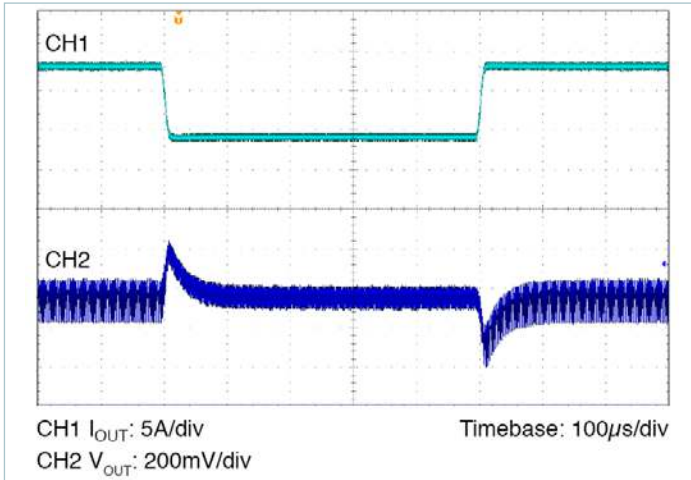
Figure 73 — Transient Response: 50% to 100% load, at 1A/μs. Nominal Line, Nominal Trim, C OUT = 8 x 10μF Ceramic
