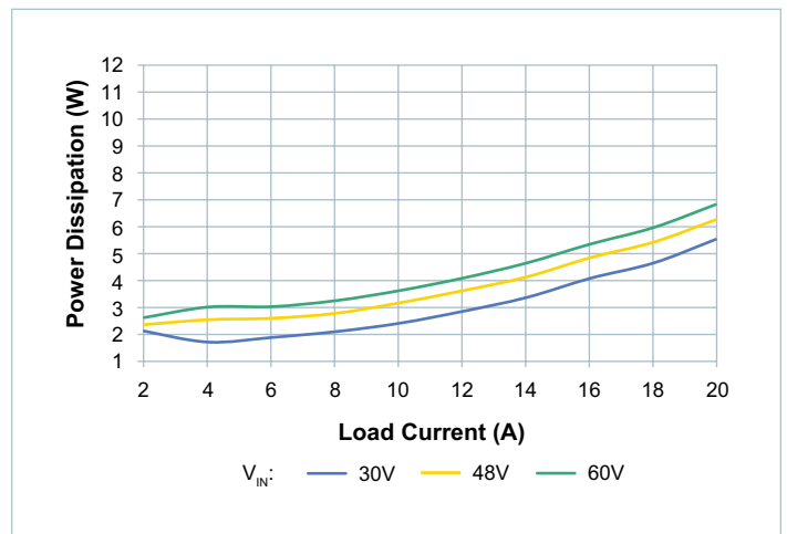
Figure 44 — System Power Dissipation, Low Trim, Board Temperature = -40°C
