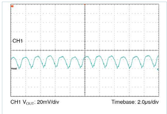
Figure 50 — Output Voltage Ripple: Nominal Line, Nominal Trim, 50% load, C OUT = 12 x 47μF Ceramic
