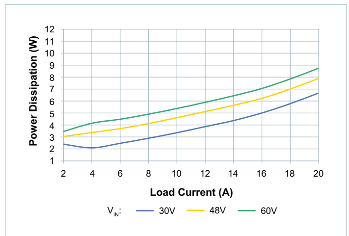
Figure 45 — System Power Dissipation, High Trim, Board Temperature = -40°C
