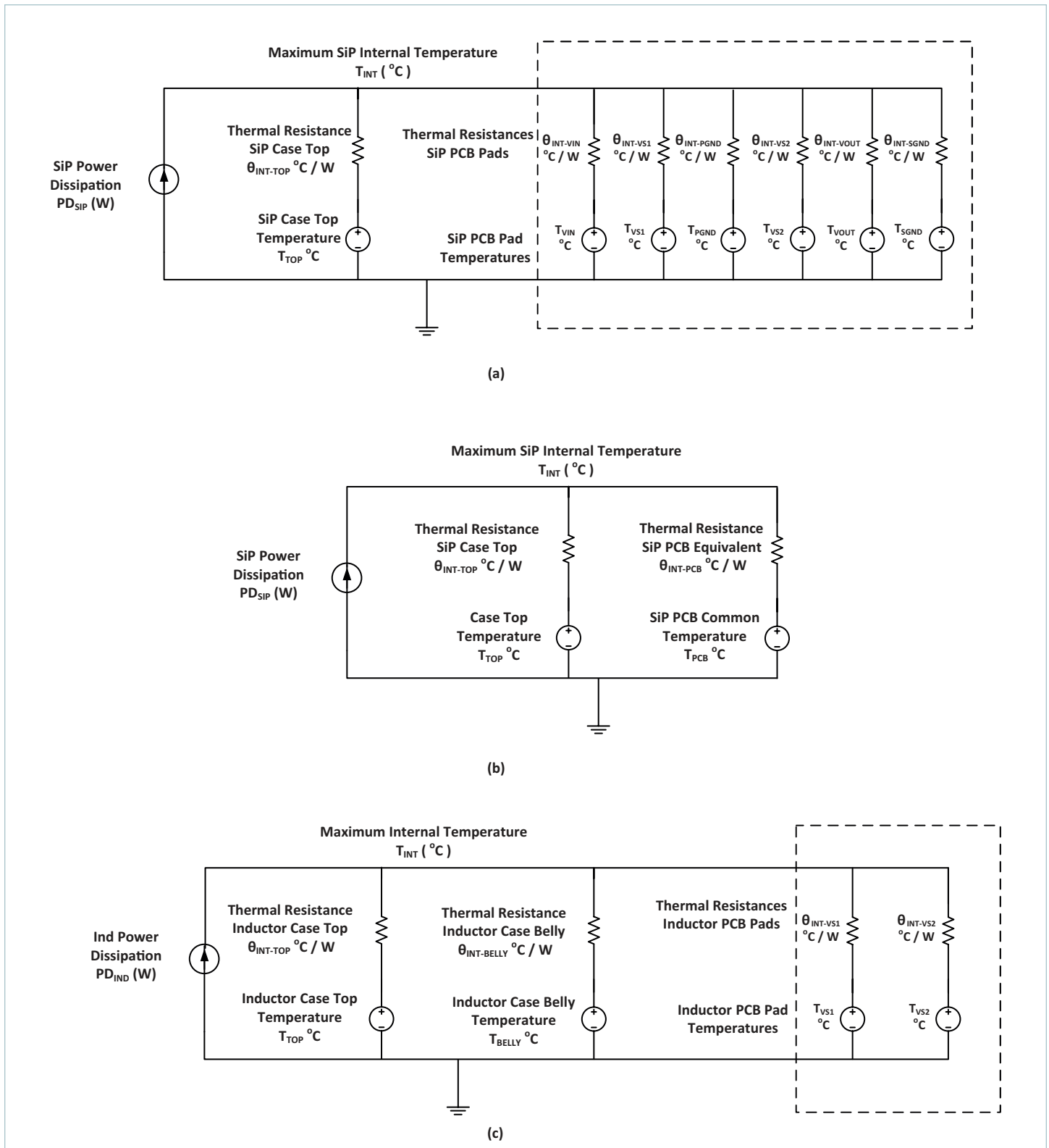
Figure 83 — PI352x-00 Thermal model (a), SiP simplified version (b) and inductor thermal model (c)
