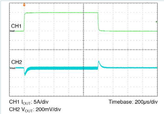
Figure 46 — Transient Response: 50% to 100% load, at 1A/μs. Nominal Line, Nominal Trim, C OUT = 12 x 47μF Ceramic
