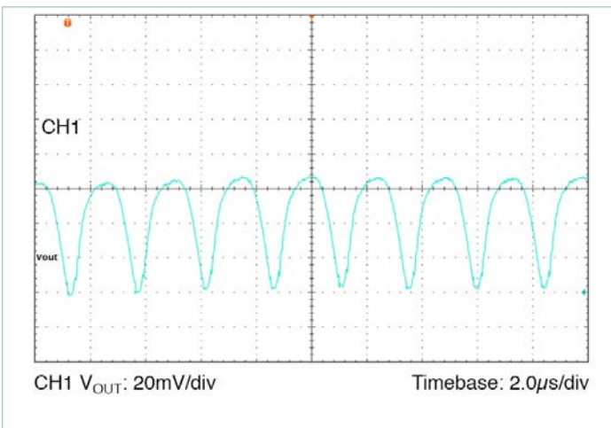
Figure 47 — Output Voltage Ripple: Nominal Line, Nominal Trim, 100% load, C OUT = 12 x 47μF Ceramic
