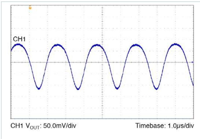
Figure 74 — Output Voltage Ripple: Nominal Line, Nominal Trim, 100% load, C OUT = 8 x 10μF Ceramic
