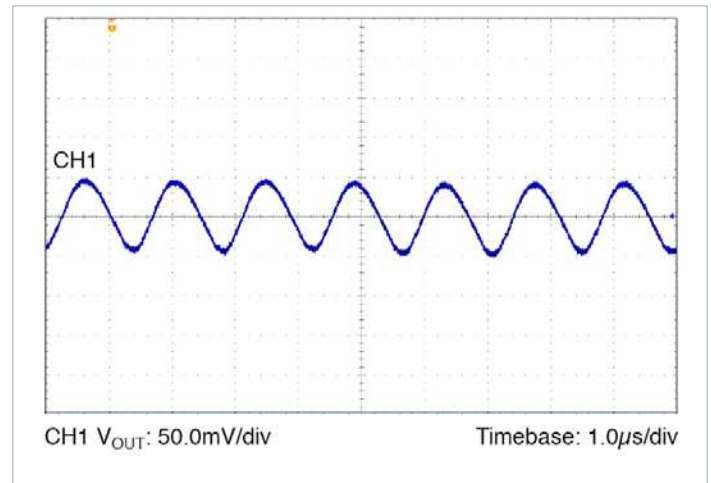
Figure 77 — Output Voltage Ripple: Nominal Line, Nominal Trim, 50% load, C OUT = 8 x 10μF Ceramic
