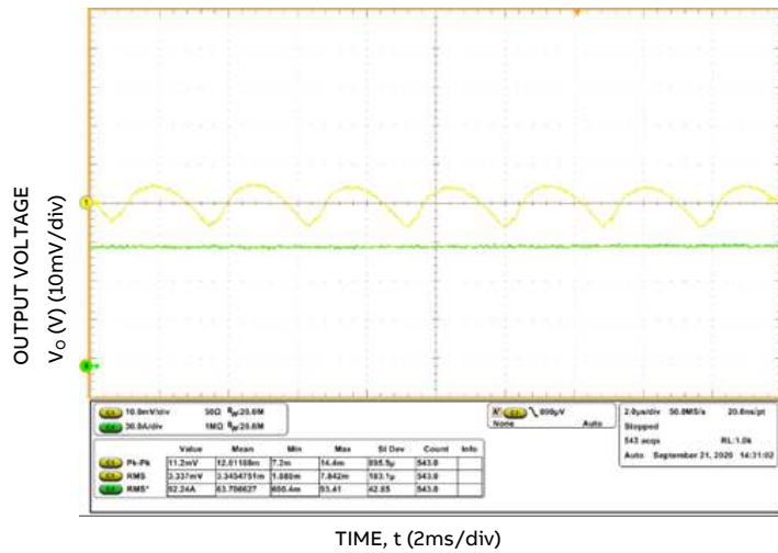
Figure 3. Typical ripple and noise ( C_o = 4 \times 22\mu F + 12 \times 47\mu F + 4 \times 680\mu F , V_{in} = 12V , I_o = I_{o,max} ).
