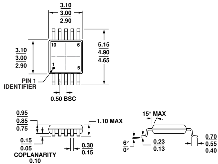
Figure 26. 10-Lead Mini Small Outline Package [MSOP]
