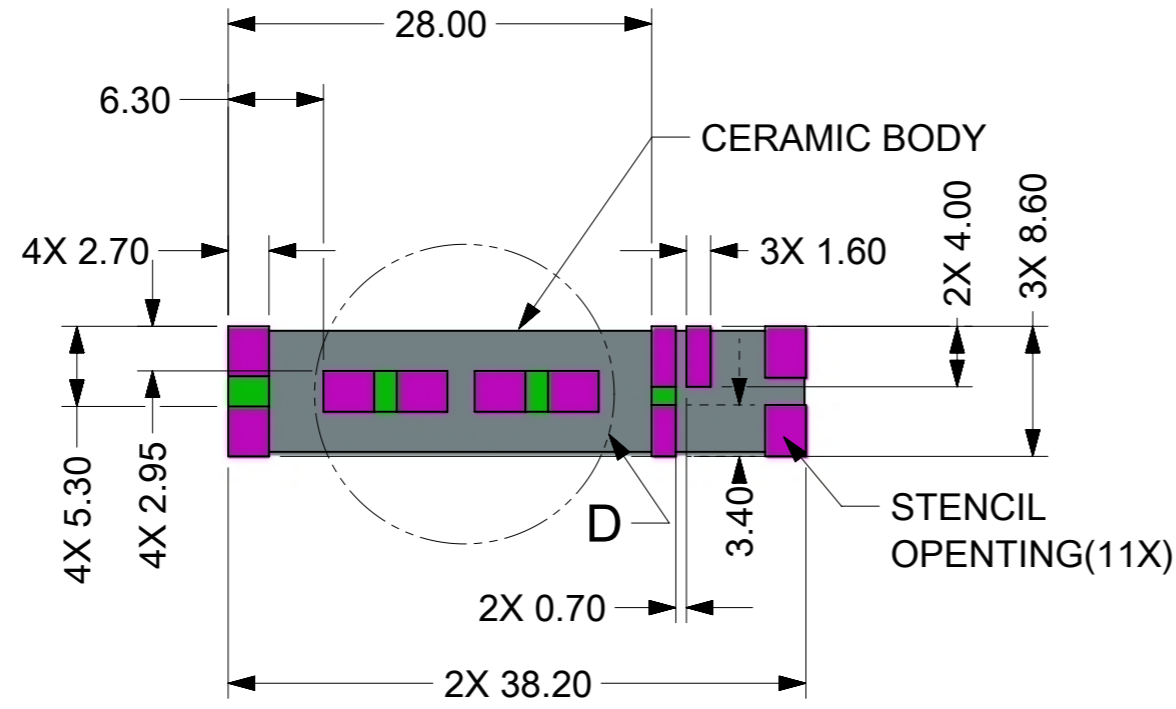
RECOMMENDED STENCIL OPENING(PINK COLOR)
