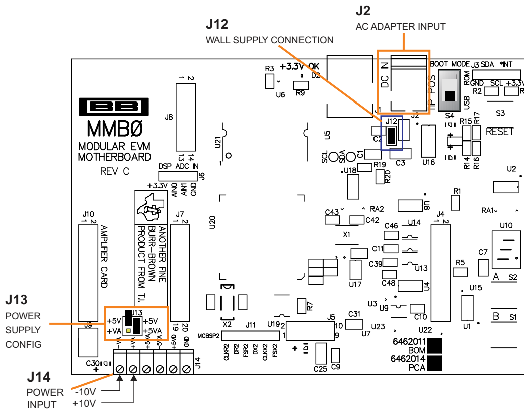
Figure 7. Using the +6V Wall Supply for +5V
