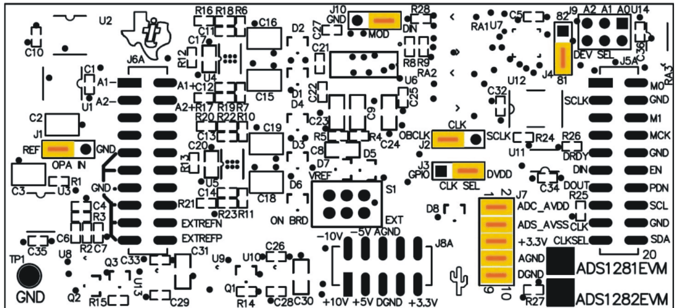
Figure 4. ADS1281EVM Default Jumper Locations
