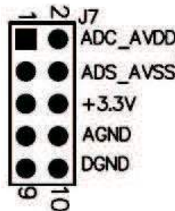
Figure 1. Connectors for J7
