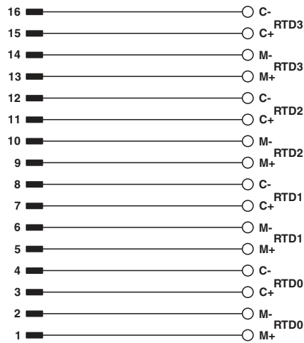
Circuit diagram
