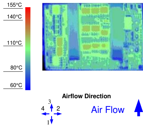
Figure 10. Thermal Image for Airflow Direction 3 (39A output, 55°C ambient, 200 LFM, typical V_{in} , open frame, soldered interface)
