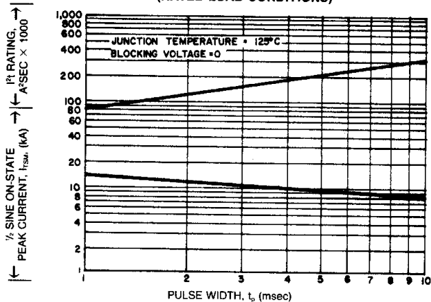
SUB-CYCLE SURGE AND I²t RATINGS (RATED LOAD CONDITIONS)
