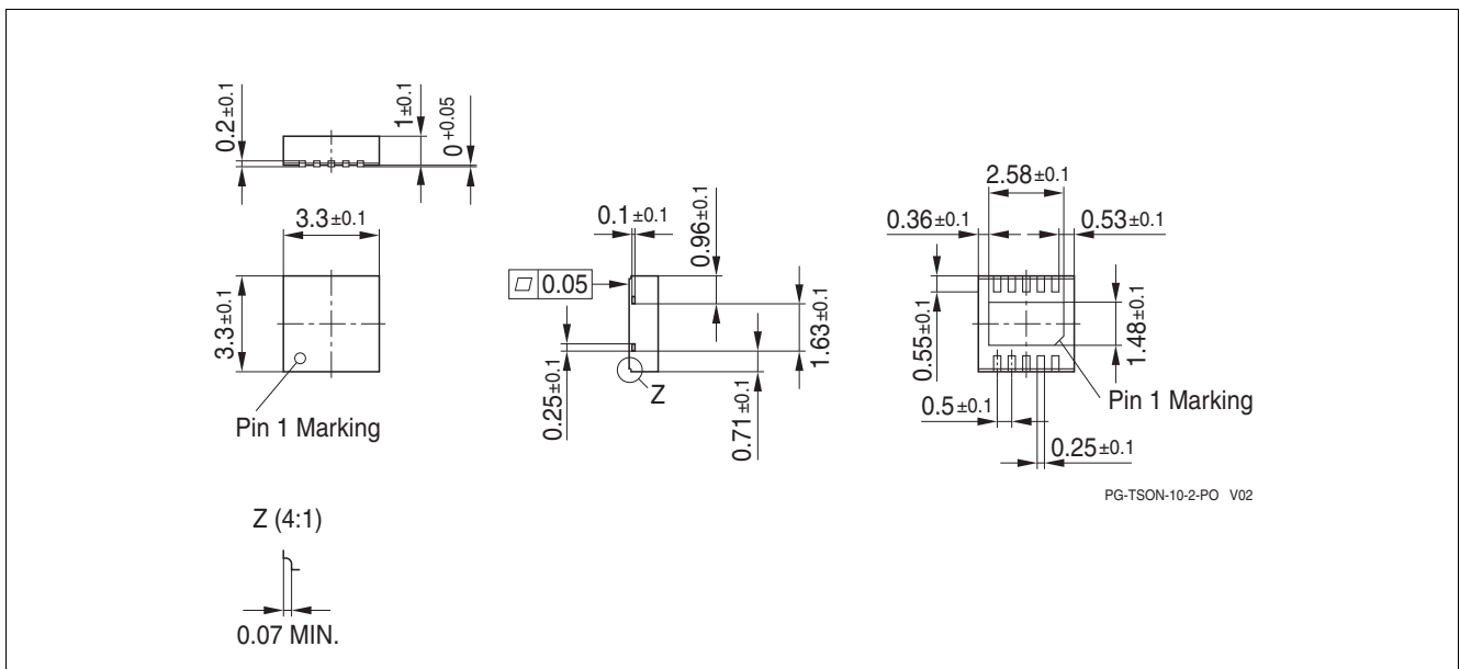
Figure 9 PG-TSON-10 Package Outlines
