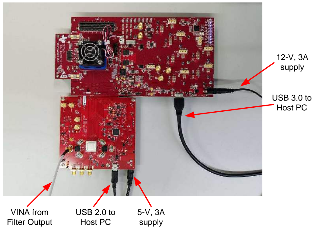
Figure 2-1. EVM Test Setup
