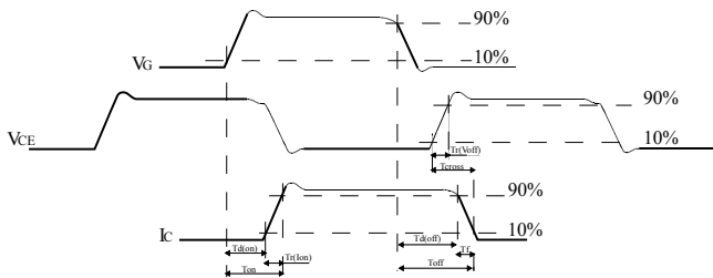
Figure 30. Switching waveform
