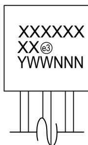
3-lead TO-92
