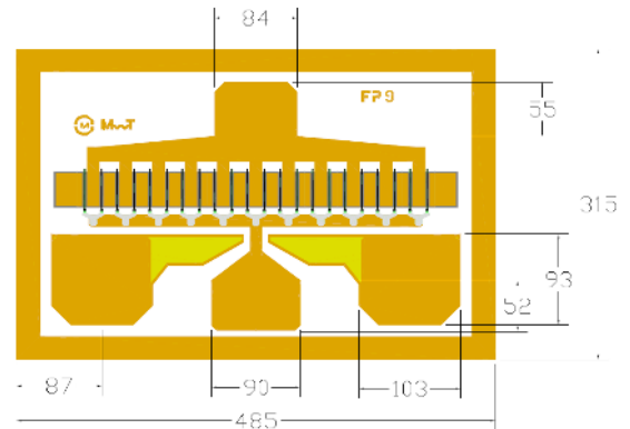
Chip Dimensions: 485 x 315 microns Chip Thickness: 100 microns
