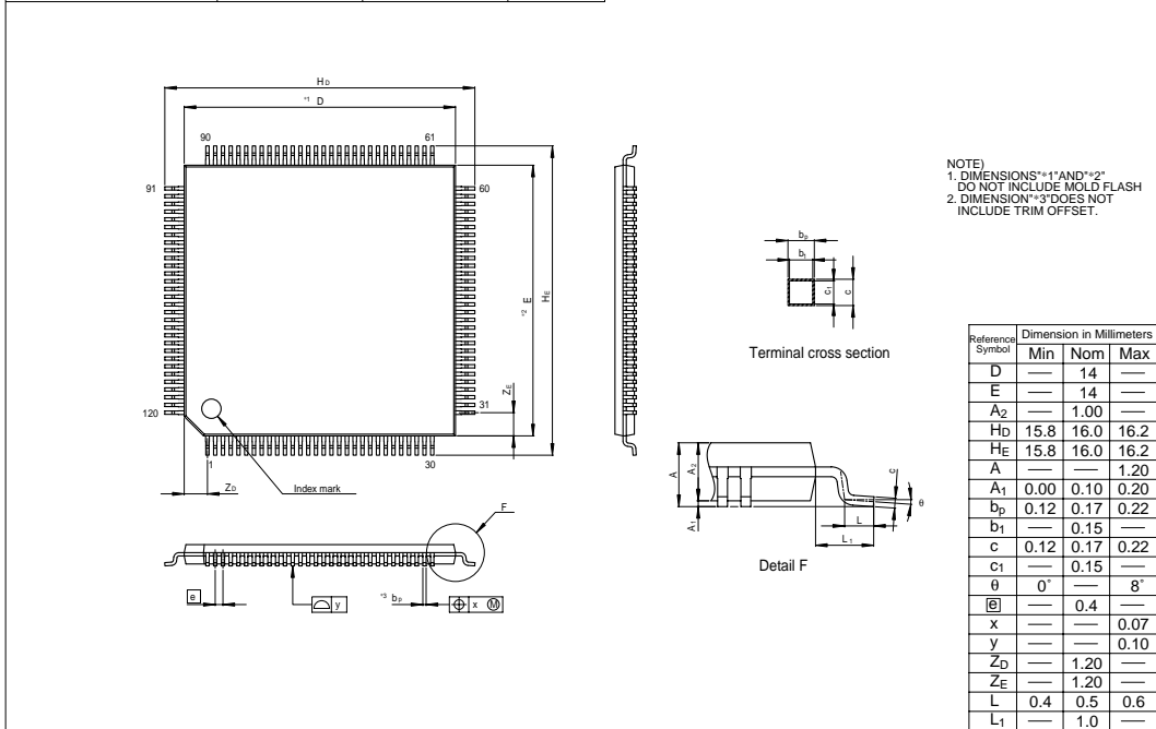
Figure C.2 Package Dimensions (PTQP0120LA-A)
