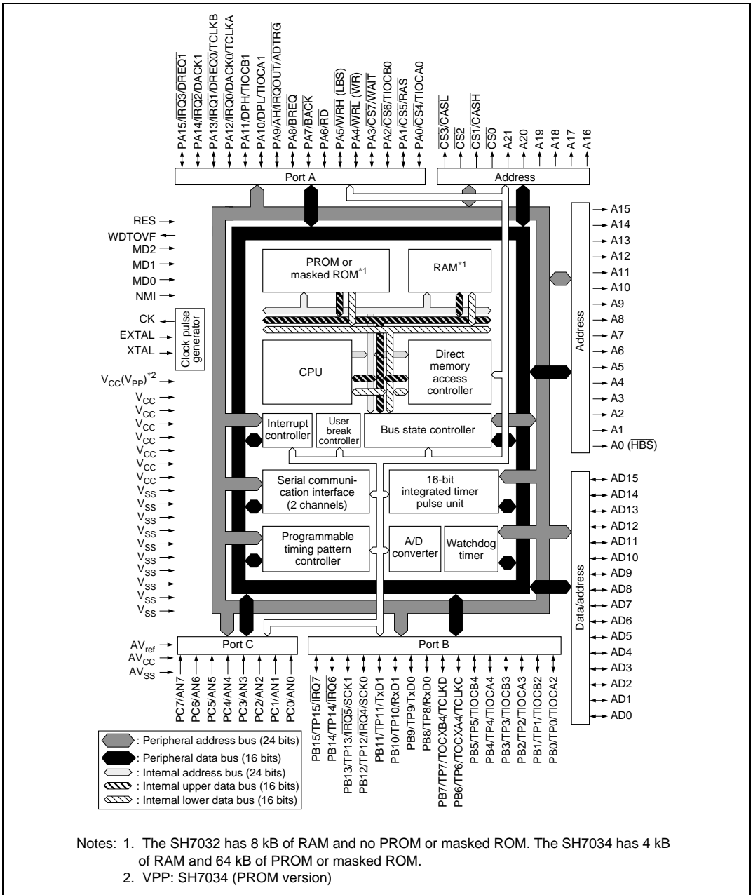
Figure 1.1 Block Diagram
