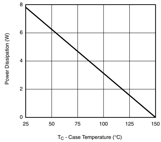
Power Derating
