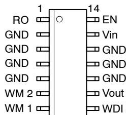
Figure 3. Pin Connections (Top View)
