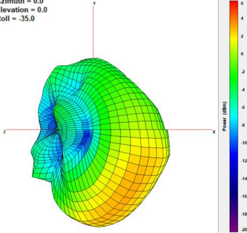
XZ Plane
