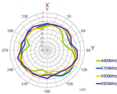
XY Plane
