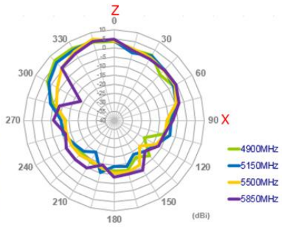
XZ Plane
