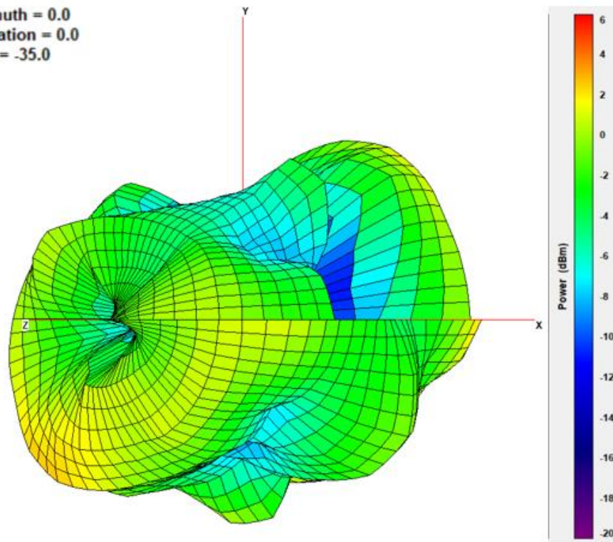
XY Plane
