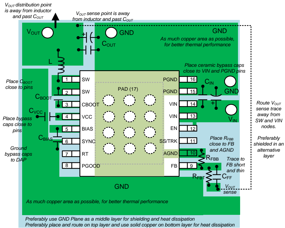
Figure 102. LM46001-Q1 PCB Layout Example
