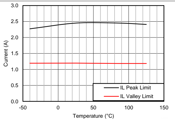
Figure 31. Peak and Valley Current Limits vs Junction Temperature
