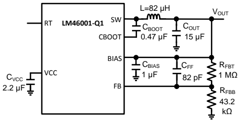
Figure 77. BOM for V_{OUT} = 24\text{ V} , F_S = 500\text{ kHz}
