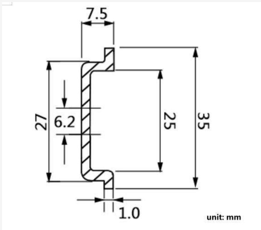
Dimension of Rail Mount Adapter
