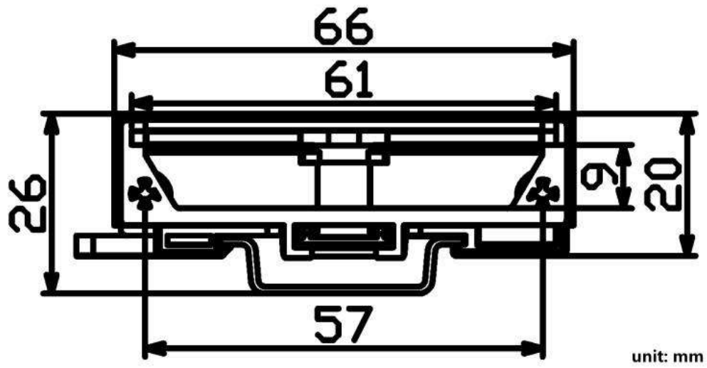
Dimension of Rail Mount Bracket
