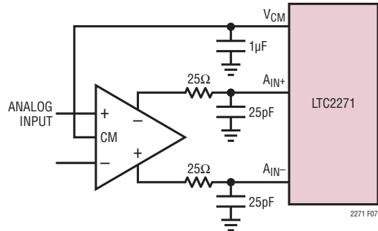
Figure 7. DC-Coupled Amplifier
