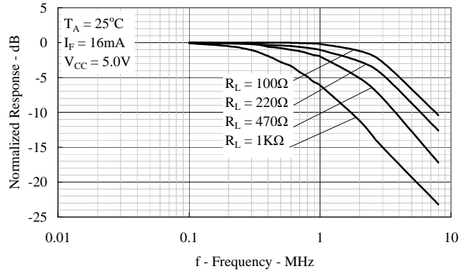
Figure 8: Frequency Response.
