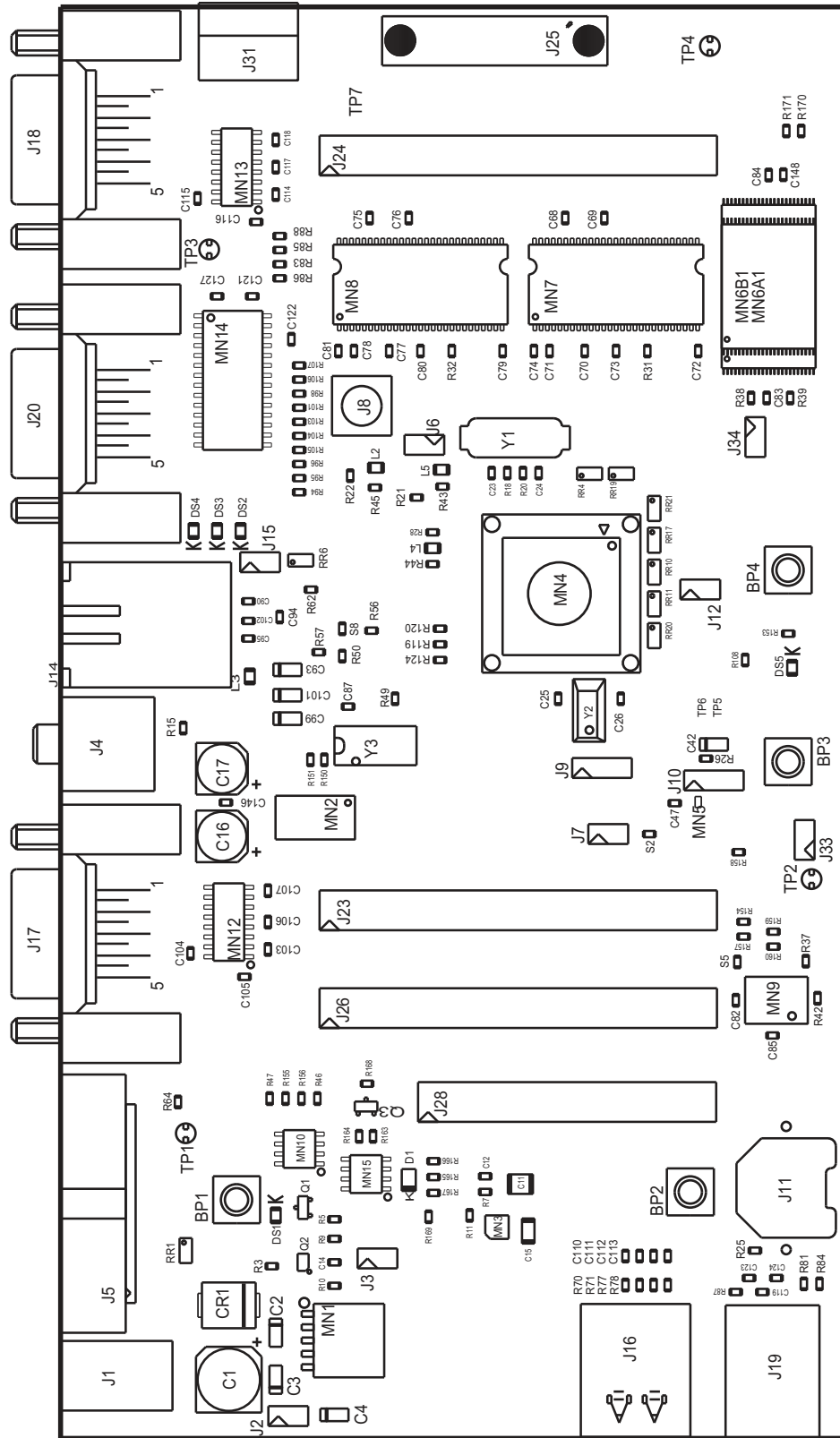
Figure 2-1. Top View
