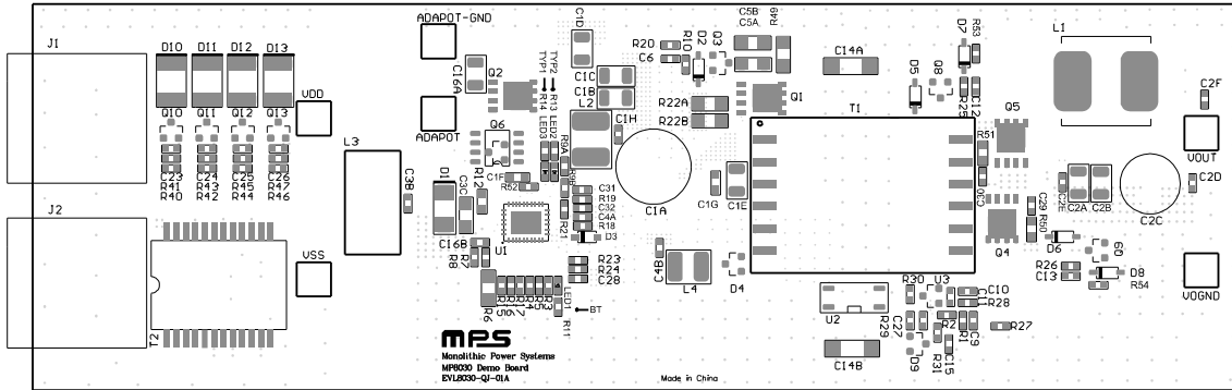
Figure 3: Top Silk
