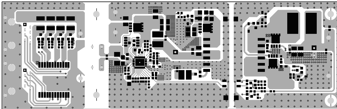
Figure 4: Top Layer
