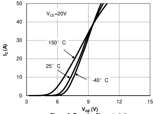
Figure 3: Transfer Characteristic
