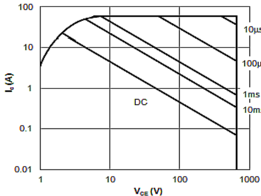
Figure 9: Forward Bias Safe Operating Area ( T_c=25^{\circ}\text{C} , V_{EE}=15\text{V} )
