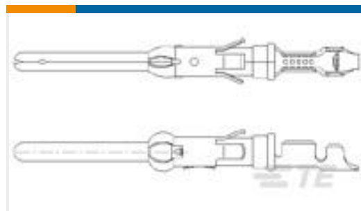
TE Part #163082-1 PIN, MALE
