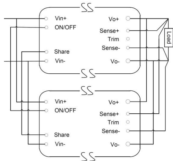
Figure 15. Circuit Configuration for Active Current Share
