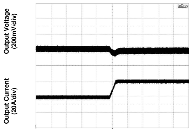
Figure 6. Transient Load Response (typical Vin, load current steps from 50% to 75% at a slew rate 0.1A/µs)
