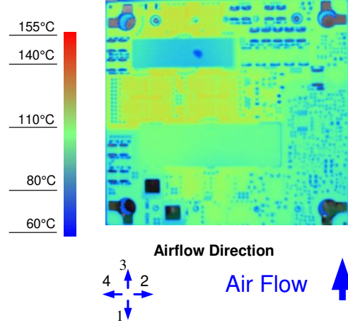
Figure 8. Thermal Image for Airflow Direction 3 (11A output, 55°C ambient, 200 LFM, typical Vin, open frame, unit soldered onto a fixture board)
