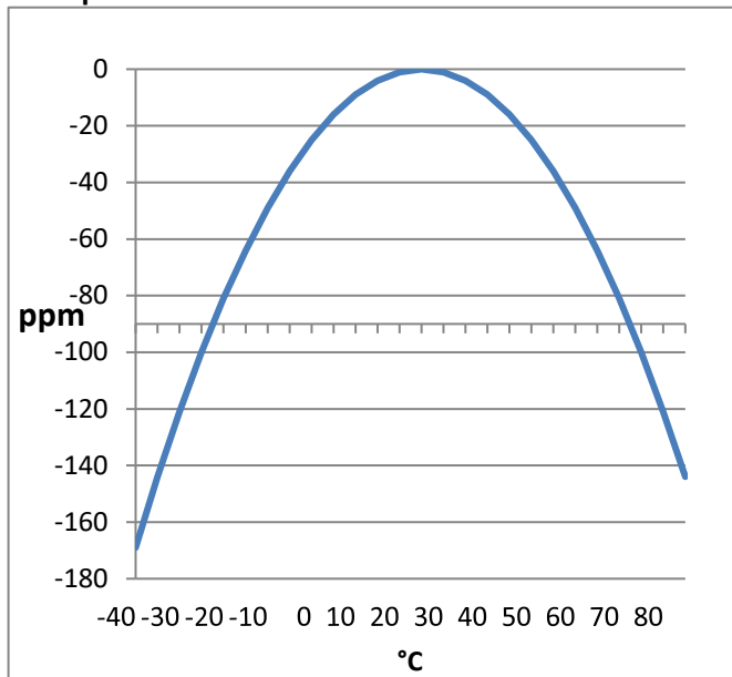
Temperature Coefficient
