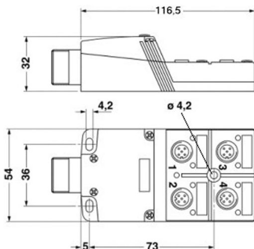
Dimensioned drawing
