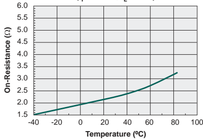
Typical On-Resistance vs. Temperature ( I_F=20\text{mA} , I_L=0.5\text{A} )
