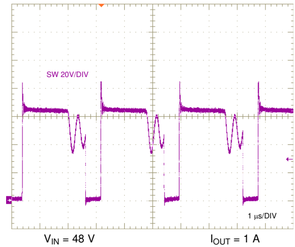
Figure 33. Switch Voltage
