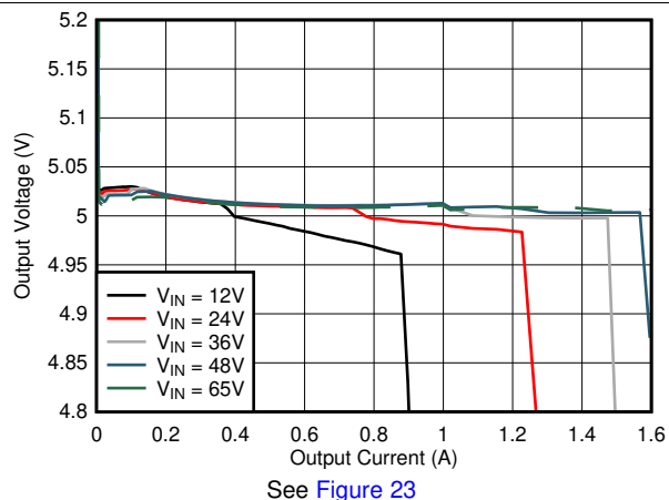
Figure 2. Output Voltage versus Load
