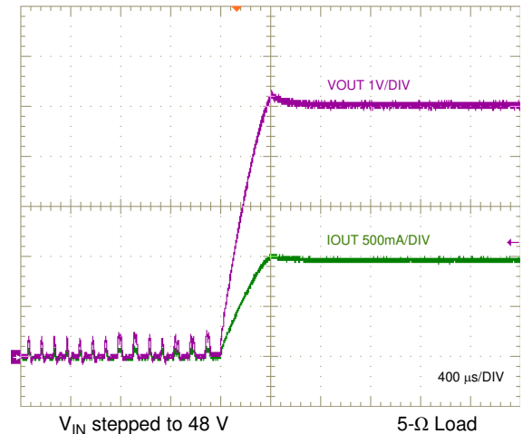
Figure 31. Short Circuit Recovery
