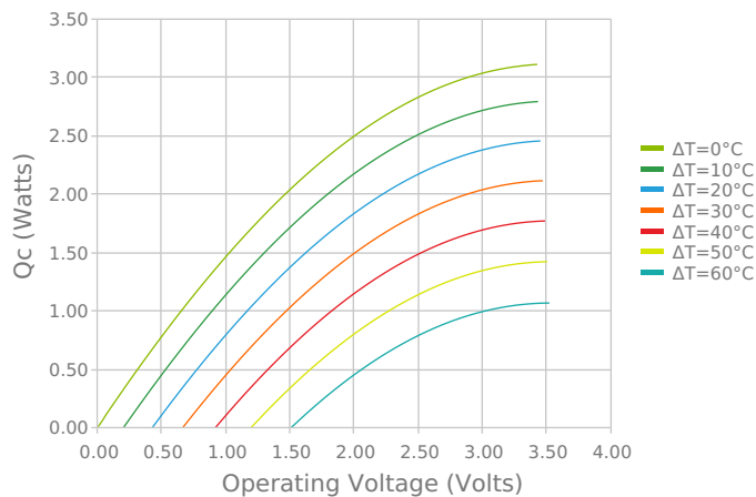
Heat Pumped at Cold Side T hot = 27 °C
