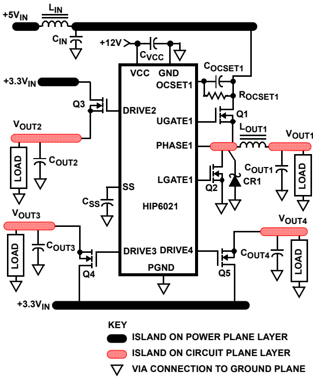
FIGURE 8. PRINTED CIRCUIT BOARD POWER PLANES AND ISLANDS
