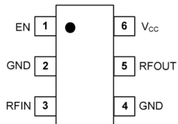
SC70-6 (C6)
