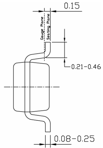
END VIEW
