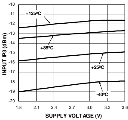
IIP3 vs Supply Voltage f_{RF} = 315\text{MHz}
