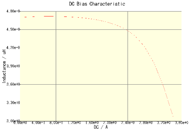
CLF6045T-4R7N-CA(Amb. Temp. = 20degc)
