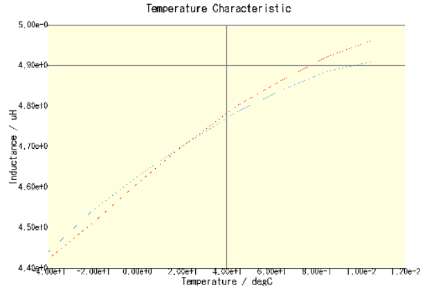
CLF6045T-4R7N-CA(DC = 0A)
