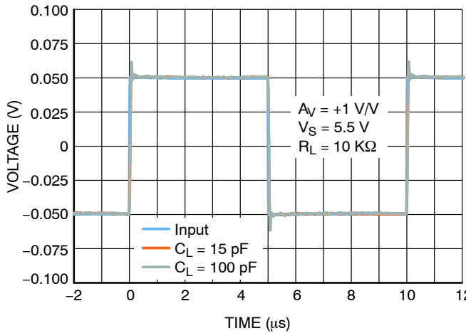
Figure 13. Non Inverting Small Signal Transient Response
